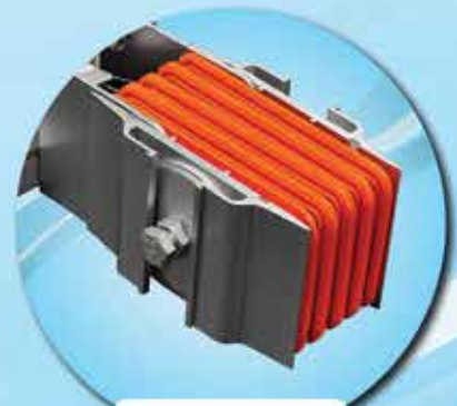
AH BUSDUCT
